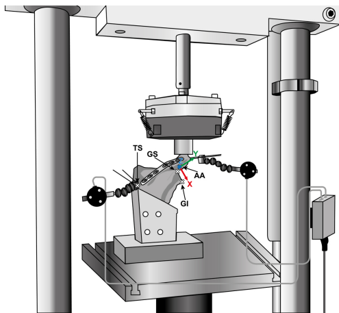
Fig. 3. Right shoulder with a single plate osteosynthesis mounted in the testing setup (GS: glenoid superior, GI: glenoid inferior; TS: trigonum scapulae; AA: acromion angle)
